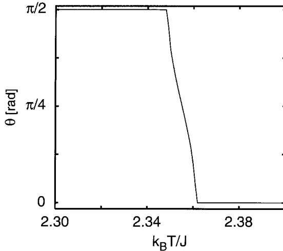
Figure 3. Variation in the angle of average magnetization for the system in figure 2.
