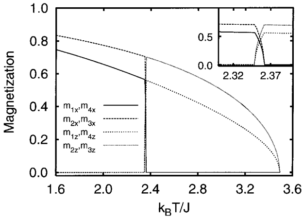
Figure 2. Normal-to-plane and in-plane components of the layer resolved magnetization for a film of four atomic layers exhibiting a reversed reorientation transition. The parameters, representative of Ni were taken from the paper by Hucht and Usadel (1997): J = 1 , \lambda_1/J = -3.5 \times 10^{-3} , \lambda_i/J = 1.5 \times 10^{-3} (i > 1) , \omega/J = 5 \times 10^{-5} . The inset shows the vicinity of the reorientation transition on an enlarged scale.
