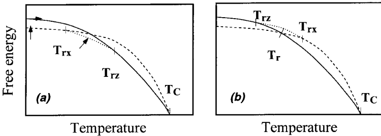
Figure 5. Schematic picture of the free energy in the case of a (a) a second-order and (b) and a first-order reorientation phase transition. As indicated by arrows, the solid, broken and dotted curves refer to the in-plane, normal-to-plane and canted mean-field solutions respectively.
