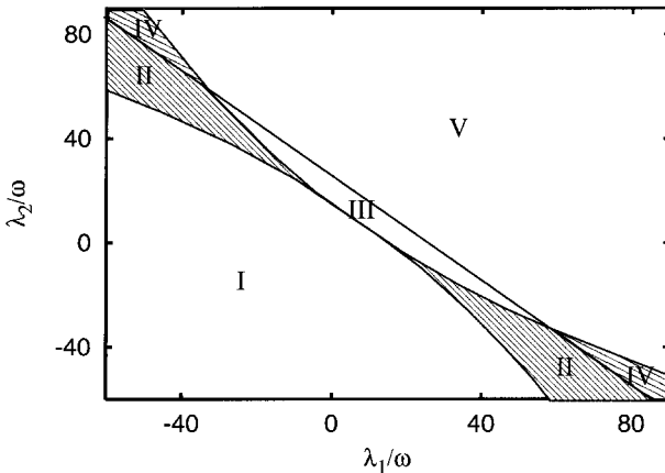
Figure 4. Phase diagram of the magnetic ground states and the reorientation phase transitions for a bilayer, where the magnetic dipole-dipole coupling strength \omega = 0.01J : region I, in-plane magnetization up to T_C ; region II, canted ground state with reorientation transition to in-plane orientation; region III, normal-to-plane ground state with reorientation transition to in-plane orientation; region IV, canted ground state with reversed reorientation transition; region V, normal-to-plane magnetization up to T_C .
