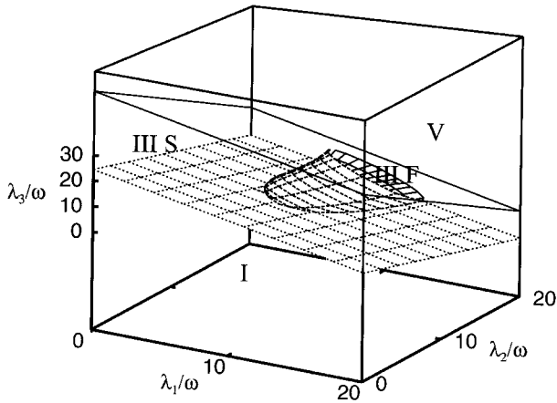
Figure 7. Mean-field phase diagram of reorientation transitions for a trilayer ( N = 3 ): region I, in-plane magnetization up to T_C ; region III S, second-order normal-to-plane to in-plane reorientation; region III F, first-order normal-to-plane to in-plane reorientation; region V, normal-to-plane magnetization up to T_C .
