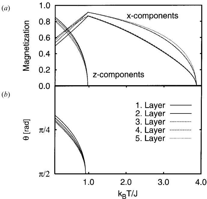
Figure 1. Out-of-plane to in-plane reorientation transition in a five-layer system ( \lambda_1/J = 0.26 , \lambda_{2,\dots,5} = 0 , \omega/J = 0.0056 ). The z and the x components of (a) the average magnetization and (b) the angles of magnetization with respect to the normal of the surface are shown.
