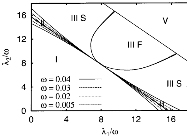
Figure 6. Phase diagram of reorientation transitions for a bilayer ( N = 2 ). Regions I, II, III and V denote the same regions as in figure 4; regime III, however, is partitioned into regions referring to first-order (III F) and second-order (III S) normal reorientation phase transitions. The corresponding boundary lines are shown for different values of the magnetic dipole-dipole interaction strength \omega , measured in units of J .
