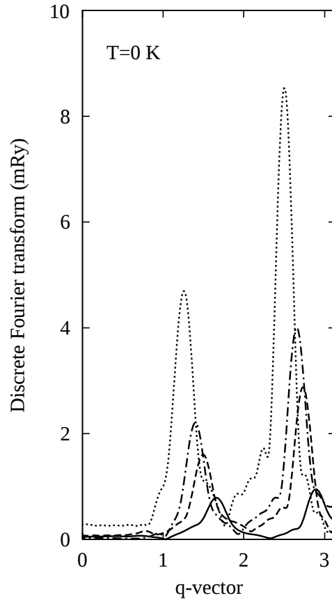
Figure 1. Composition dependence of the absolute values of a discrete Fourier transform of \bar{\mathcal{E}}_x at T = 0 K for two Co(001) slabs each five monolayers thick separated by an fcc-Cu 1-x Ni x alloy spacer: (i) Cu 0.75 Ni 0.25 (full line); (ii) Cu 0.85 Ni 0.15 (dashed line); (iii) Cu 0.9 Ni 0.1 (dashed-dotted line); and (iv) an ideal Cu spacer (dotted line).
