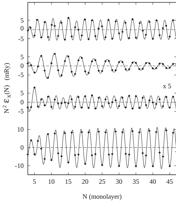
Figure 3. Exchange coupling N^2 \bar{\epsilon}_x(N) at T = 0 K as a function of the spacer thickness N for two semi-infinite Co(001) subsystems sandwiching a spacer of (from bottom to top) ideal Cu, \text{Cu}_{0.75}\text{Ni}_{0.25} (multiplied by a factor of 5), \text{Cu}_{0.5}\text{Zn}_{0.5} , and \text{Cu}_{0.5}\text{Au}_{0.5} . Diamonds refer to the calculated values; the full line (Fourier back-transform) serves as a guide to the eye.
