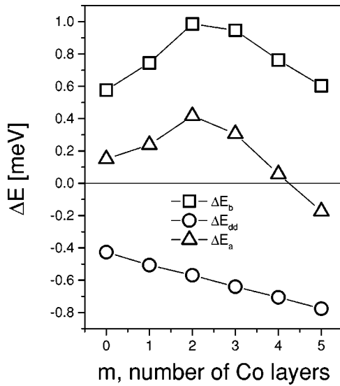
FIG. 3. Calculated band energy, \Delta E_b and magnetic dipole-dipole energy contributions, \Delta E_{dd} to the total magnetic anisotropy energy, \Delta E_a in Cu(100)/Ni 13 (-5.5%)/Ni 17 (0%)/Co m .
