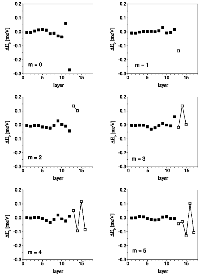
FIG. 2. Layer resolved band energy difference \Delta E_b^n for free surfaces of 0 to 5 Co layers on Ni(100)/Ni 12 (0%). Full and open squares denote Ni and Co layers, respectively.
