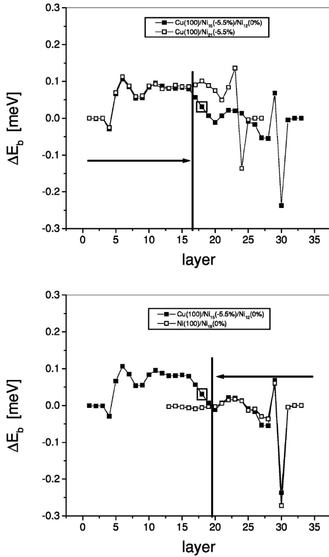
FIG. 1. Comparison of the layer-resolved band energy contributions \Delta E_b^n of Cu(100)/Ni 15 (-5.5%)/Ni 12 (0.0%) (system A, squares) with Cu(100)/Ni 21 (-5.5%) (system B, open squares, top), and in Ni(100)/Ni 18 (system C, open squares, bottom). In all cases the first layers to the right denote vacuum layers. In the case of system A the first three layers to left refer to Cu layers. The view from the Cu/Ni and from the Ni/Vac interface is indicated by arrows. The small boxes denote the last relaxed Ni layer in system A.
