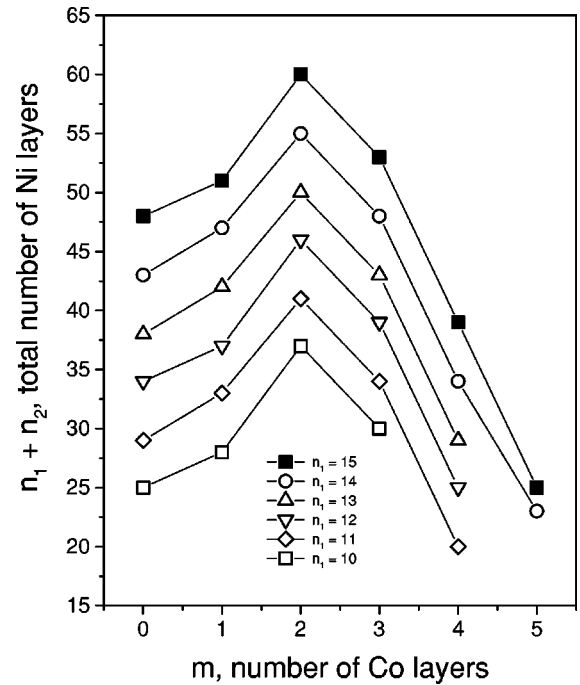
FIG. 4. Total number of Ni layers ( n_1 + n_2 ) at which the magnetic anisotropy energy, \Delta E_a of Cu(100)/Ni n 1 (-5.5%)/Ni n 2 (0%)/Co m changes sign, displayed as a function of the number of Co layers ( m ).
