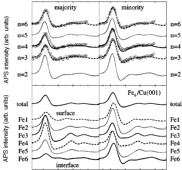
FIG. 3. Same as Fig. 2, but for the (stable) AFM configurations.
