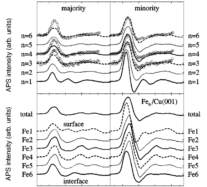
FIG. 2. Spin-resolved APS spectra for Fe in the FM ordered systems \text{Fe}_n/\text{Cu}(001) . The top panels give the total spectra for n=1, \dots, 6 for the majority (left) and minority (right) channels. In addition to the theoretical spectra based on Eq. (1) corresponding experimental data are given by open circles (Refs. 3,14). The lower panels of the figure give a layer by layer decomposition of the spectrum for n=6 with the weighting factors omitted [see Eq. (2)].
