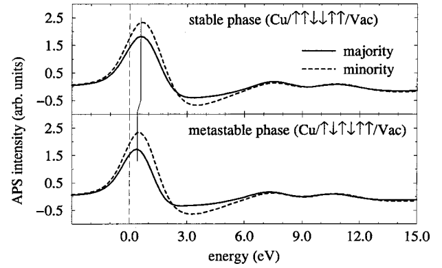
FIG. 4. Comparison between the theoretical SR-APS spectra of the stable (upper panel) and metastable (lower panel) AFM configurations of \text{Fe}_6/\text{Cu}(001) .
