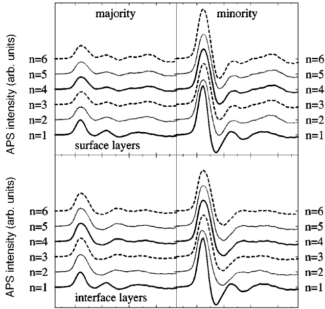
FIG. 1. Spin-resolved APS spectra for Fe in the FM ordered systems \text{Fe}_n/\text{Cu}(001) . The top panels give the spin-resolved spectra for the topmost Fe layer, while the bottom panels give the corresponding spectra for the Fe interface layer for n=1, \dots, 6 .
